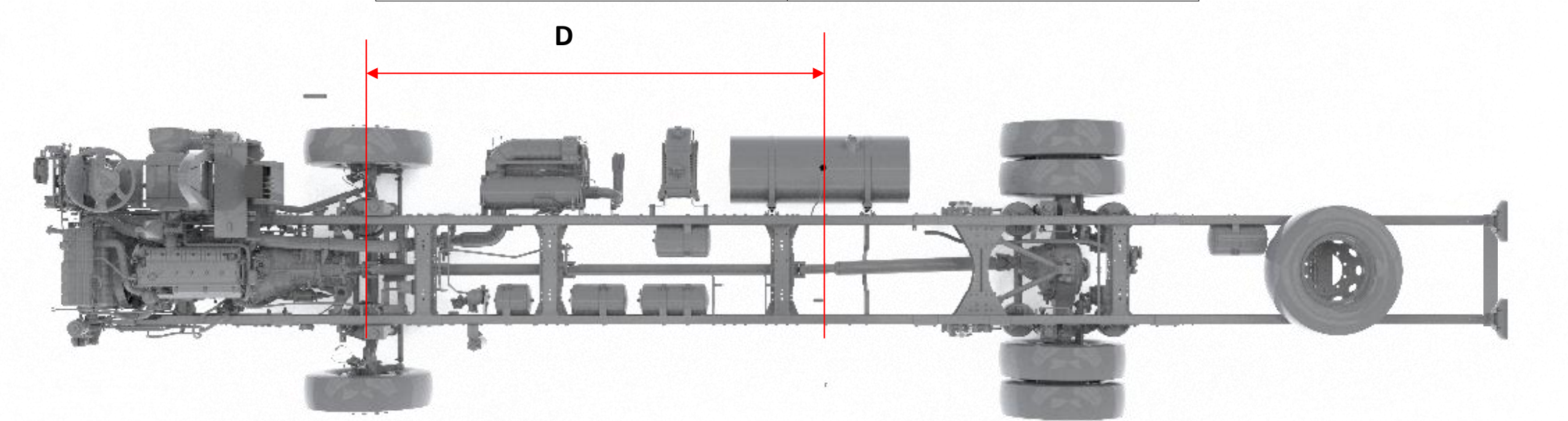
OF 1824 / 1924 Position of the reservoirs
