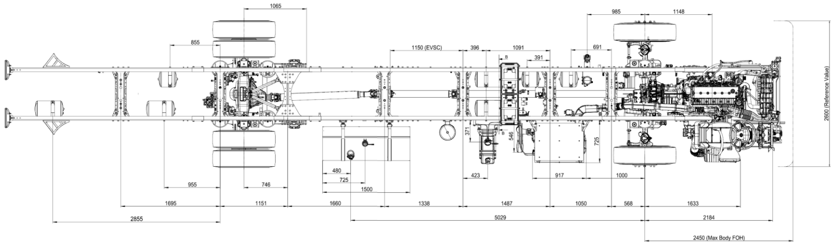
Coach Builder Drawing OF1824
