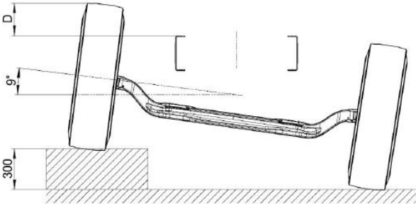
Front Axle
