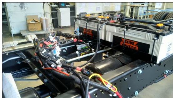
Power Distribution Board Main fuse box (1X 150A)
