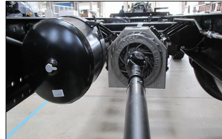
Retarder
