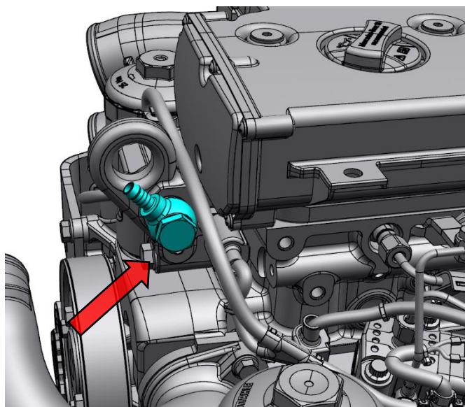
Arrangement of the space heating tap
