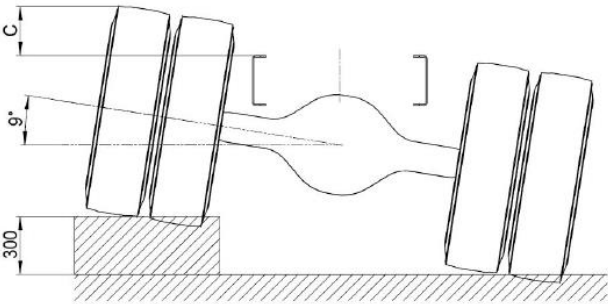
Rear Axle
