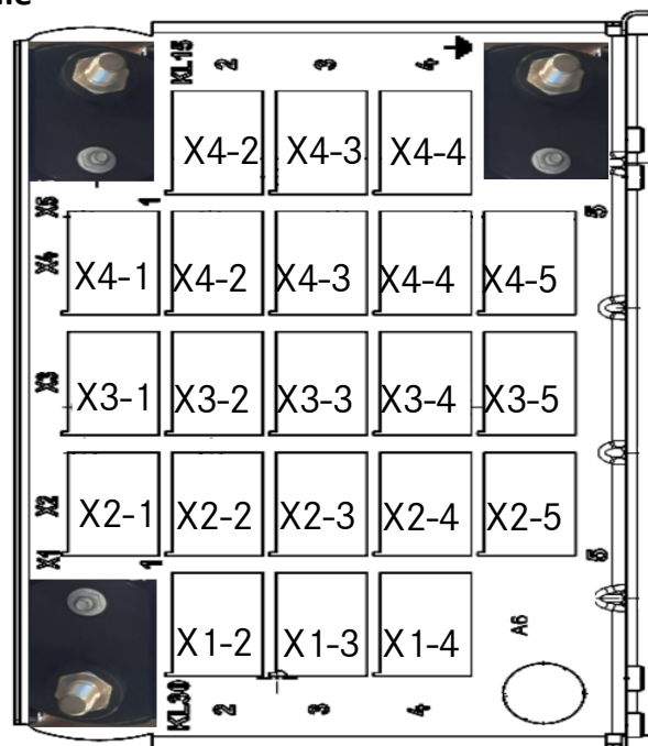
Interconnector Board connectors position
