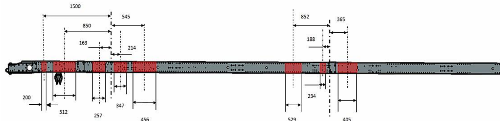
OF chassis Unsuitable areas for fastening
